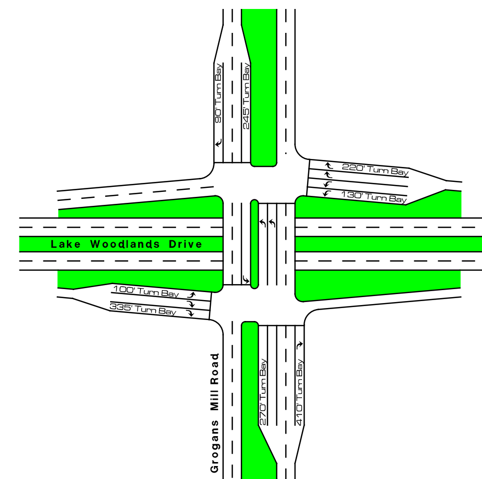
Lake Woodlands Drive 2030 Tight Diamond
