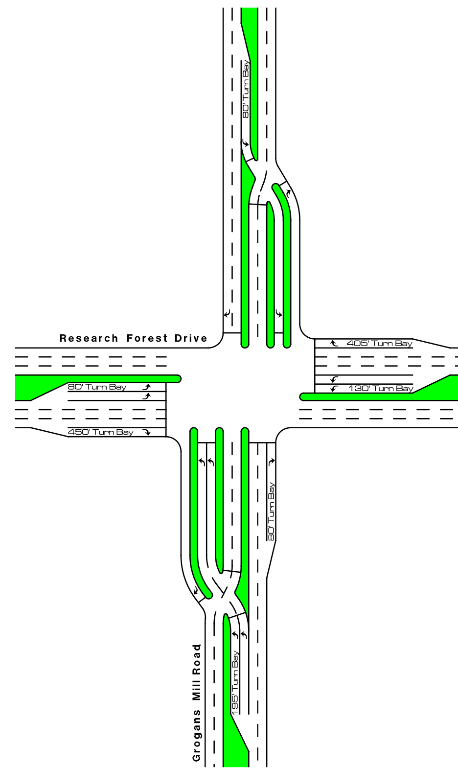
Research Forest Drive 2030 Partial Displaced Left-Turn
