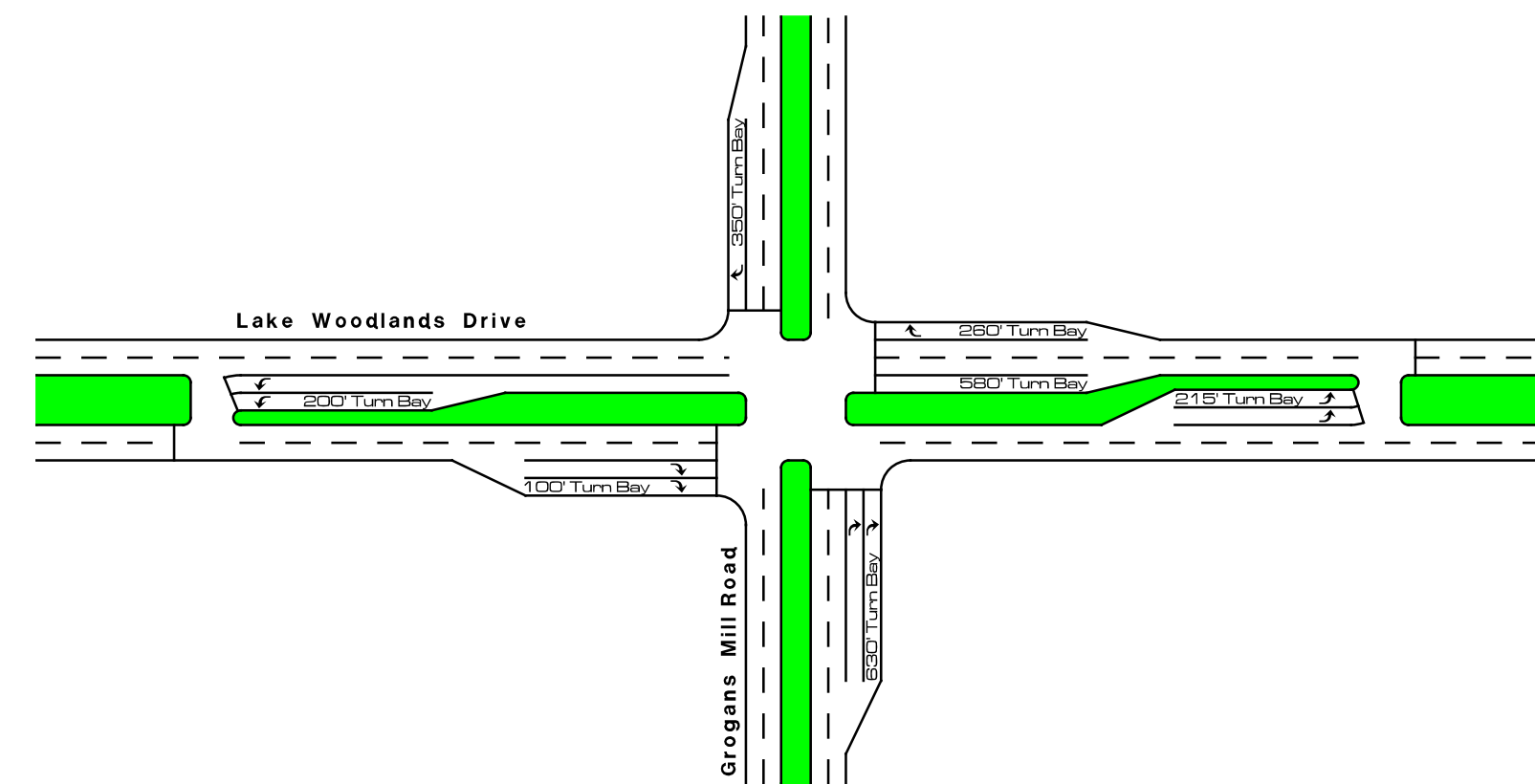
Lake Woodlands Drive 2030 Median U-Turn
