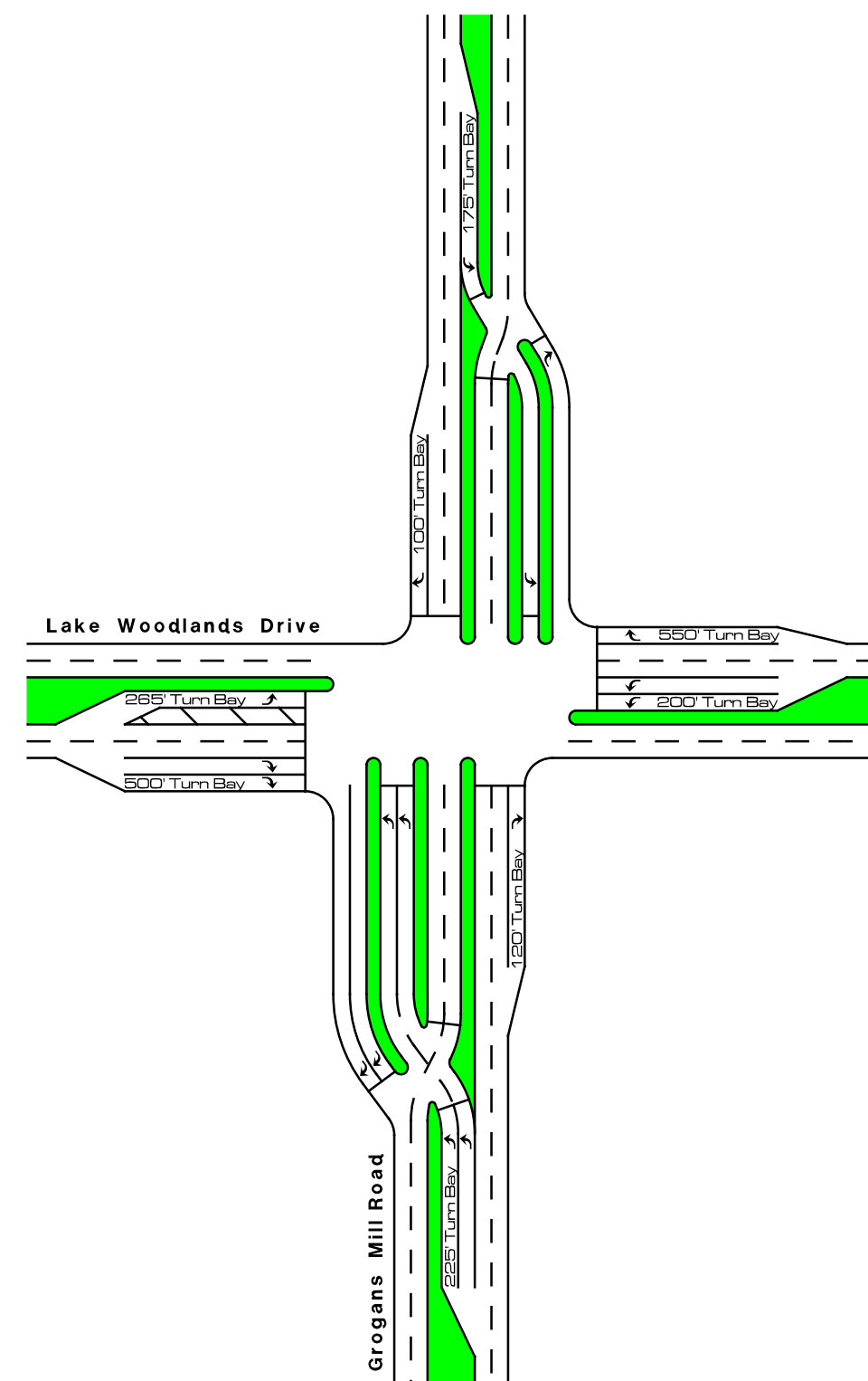
Lake Woodlands Drive 2030 Partial Displaced Left-Turn
