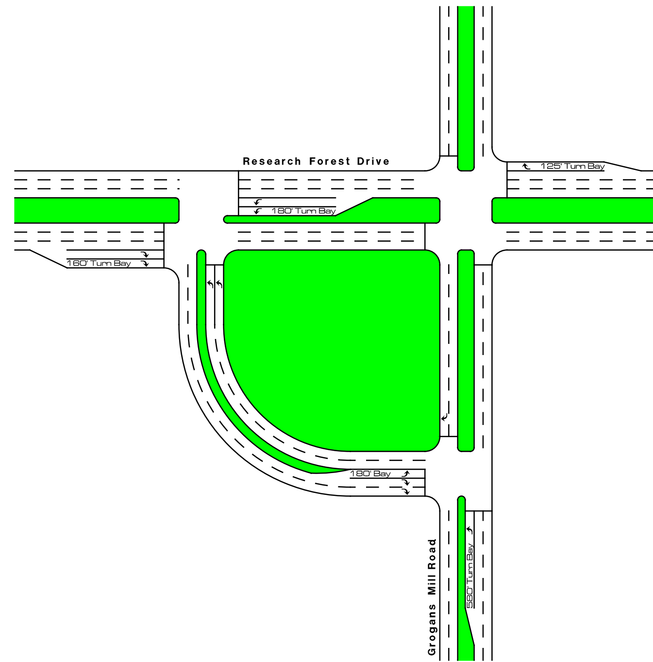
Research Forest Drive 2030 Quadrant Roadway
