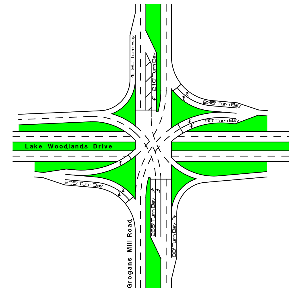
Lake Woodlands Drive 2030 Single Point
