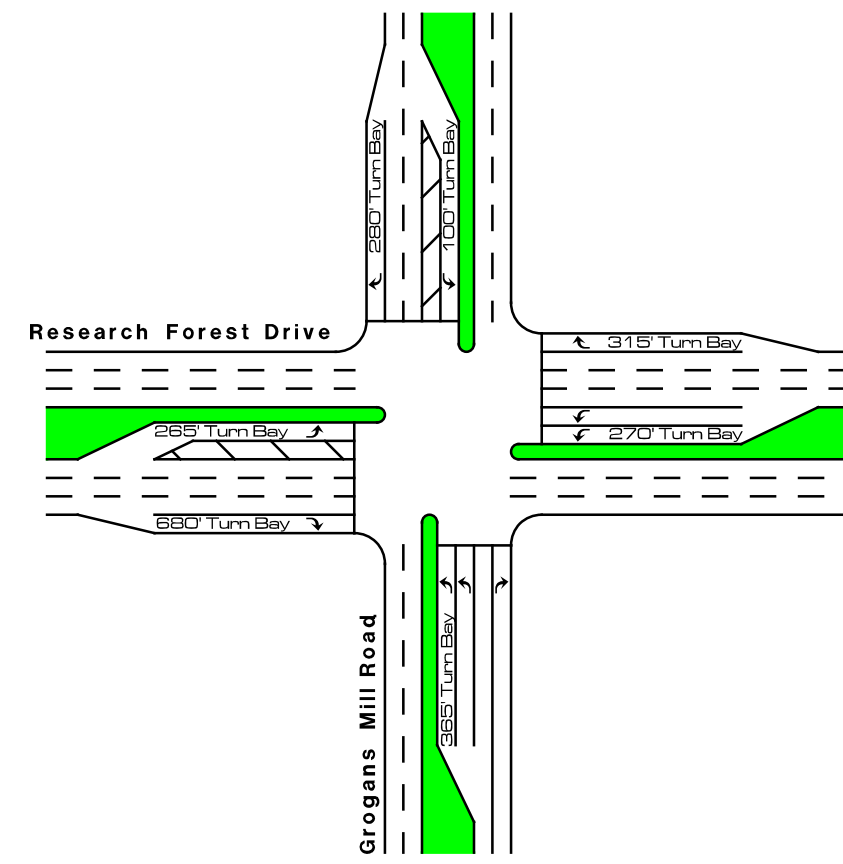
Research Forest Drive 2030 Traditional Improvement
