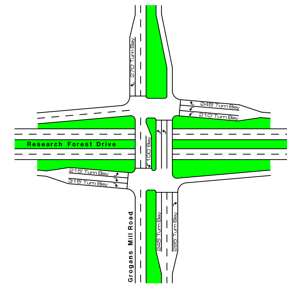
Research Forest Drive 2030 Tight Diamond
