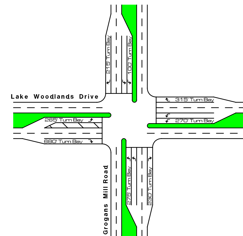
Lake Woodlands Drive 2030 Traditional Improvement
