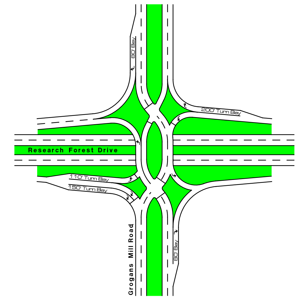
Research Forest Drive 2030 Diverging Diamond
